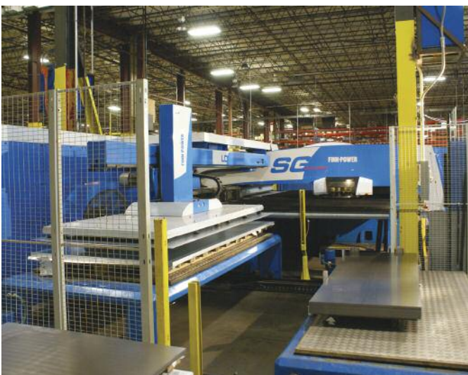
With the Shear Genius integrated punch/right angle shear combination concept, the objective is to provide one machine capable of transforming a full-sized sheet into punched parts.
